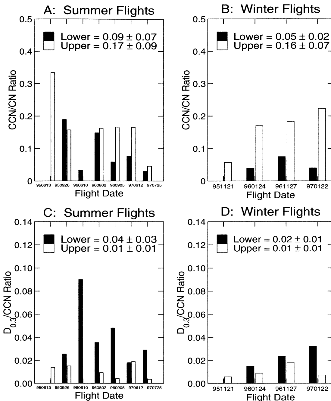
Figure 4. Aerosol ratios, CCN/CN for (a) Summer and (b) winter and D_{0.3} /CCN for (c) summer and (d) winter flights, at Laramie, Wyoming. The average and standard deviation for the lower tropospheric and upper tropospheric layers are displayed in the legends. The aerosol ratios are computed by averaging aerosol measurements within a layer and then taking the ratio of the aerosol averages.
