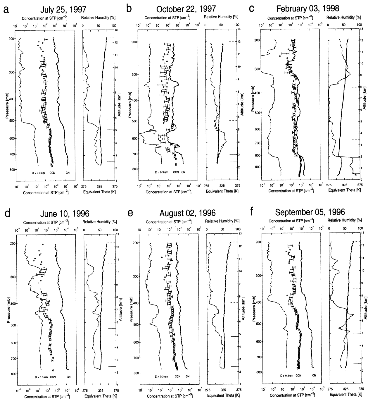
Figure 2. Vertical profiles of particles with diameter > 0.3 \mu\text{m} ( D>0.3 \mu\text{m} , thin line), CCN concentration (1% supersaturation, circles), and condensation nucleus (CN) concentration ( D>0.01 \mu\text{m} , thick line) at (a) July 25, 1997; (b) October 22, 1997; (c) February 3, 1998; (d) June 10, 1996; (e) August 2, 1996; and (f) September 5, 1996. Open circles represent measurements below the detection limit of the CCN counter. The concentration measured by each aerosol instrument has been corrected to standard temperature and pressure (STP). Equivalent potential temperature (thick line) and relative humidity (thin line) are shown at right. The left axis denotes the measured atmospheric pressure, and the far right axis denotes the altitude above mean sea level. The surface at Laramie, Wyoming, is at \sim 2.2 \text{ km} above mean sea level. The horizontal lines on the far right of the equivalent potential temperature plots denote the lower (solid lines) and upper (dashed lines) tropospheric layers. All profiles shown were obtained shortly after sunrise, usually with clear skies and light surface winds. The February 3, 1998, profile is from Lauder, New Zealand. The other five profiles are from Laramie, Wyoming.
